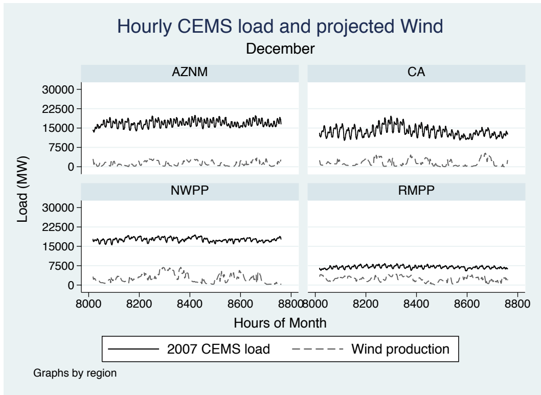
Figure 3: Hourly Load and Wind Production for December
