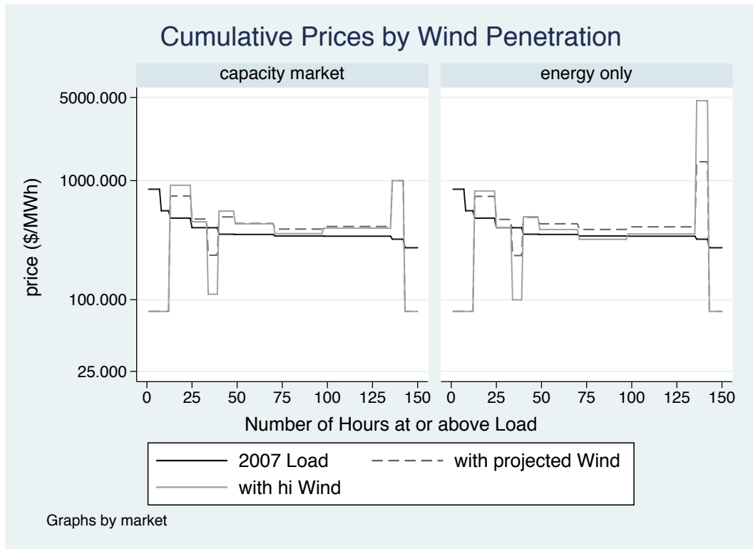
Figure 9: Peak Hour Prices for RMPP
