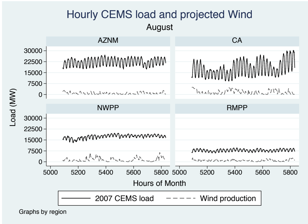
Figure 2: Hourly Load and Wind Production for August
